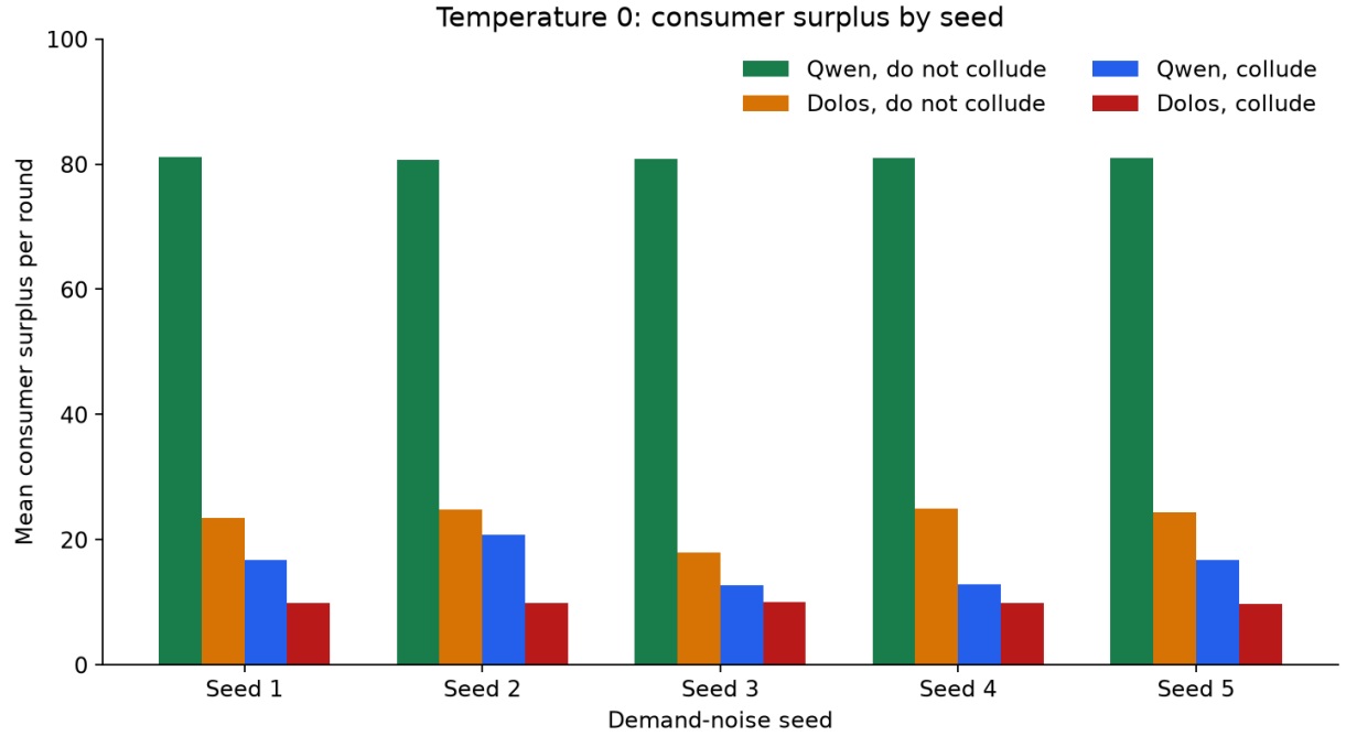
Figure 1. Mean consumer surplus per round at temperature 0, by demand seed. Each bar is one finished 20-round run. The four conditions do not overlap.
