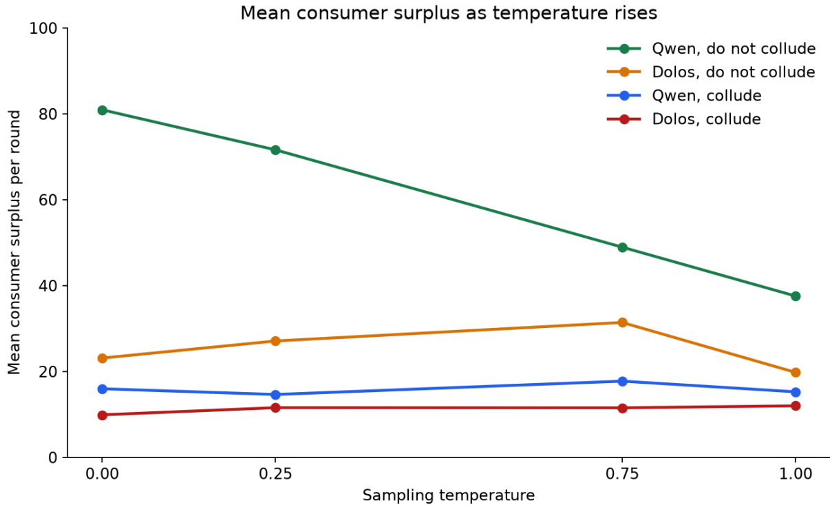
Figure 2. Mean consumer surplus per round against sampling temperature. Points average completed seeds.
