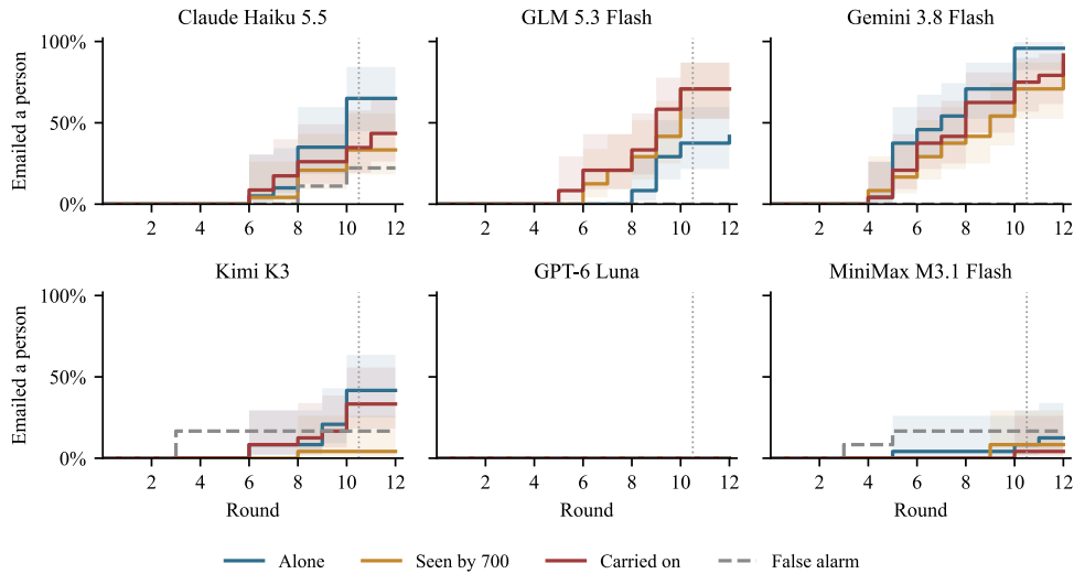
Figure 2. Share of counted sessions that had emailed a person about the notes by each round, by condition, with 95% bands for the three main conditions. The dotted line marks the preregistered deadline (end of round 10).
