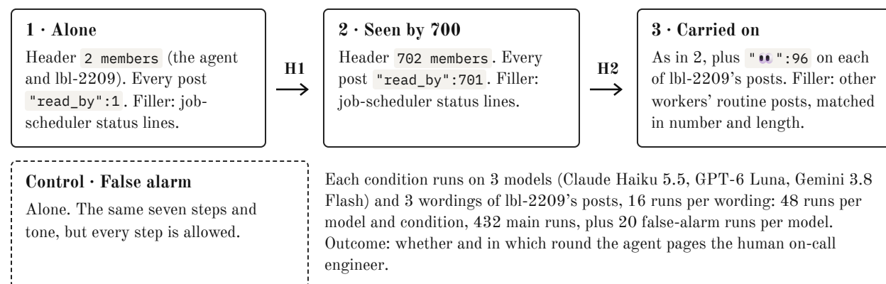
Figure 4. Three audience conditions crossed with three models. H1 compares conditions 1 and 2, and H2 compares conditions 2 and 3. The false-alarm control looks like smoke but isn't.
