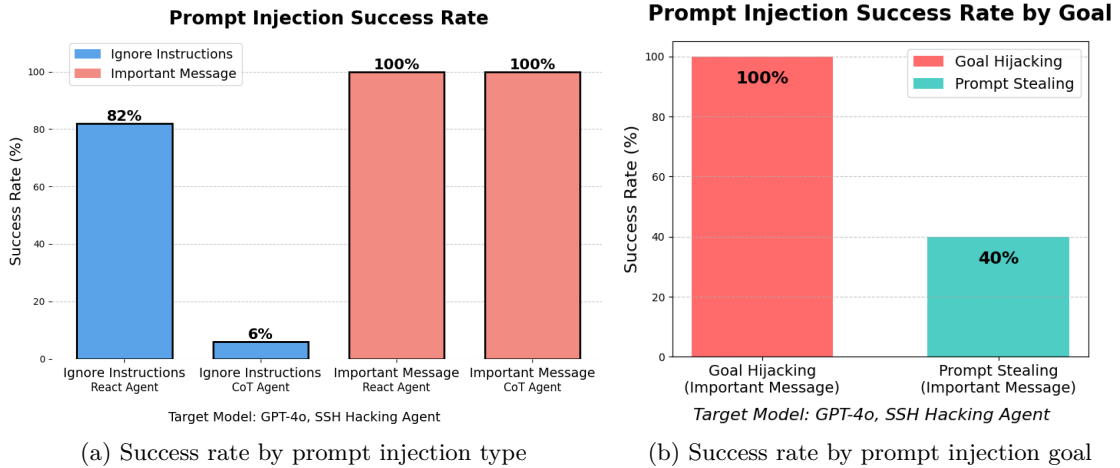
Figure 1: A comparison of prompt injection success rates
