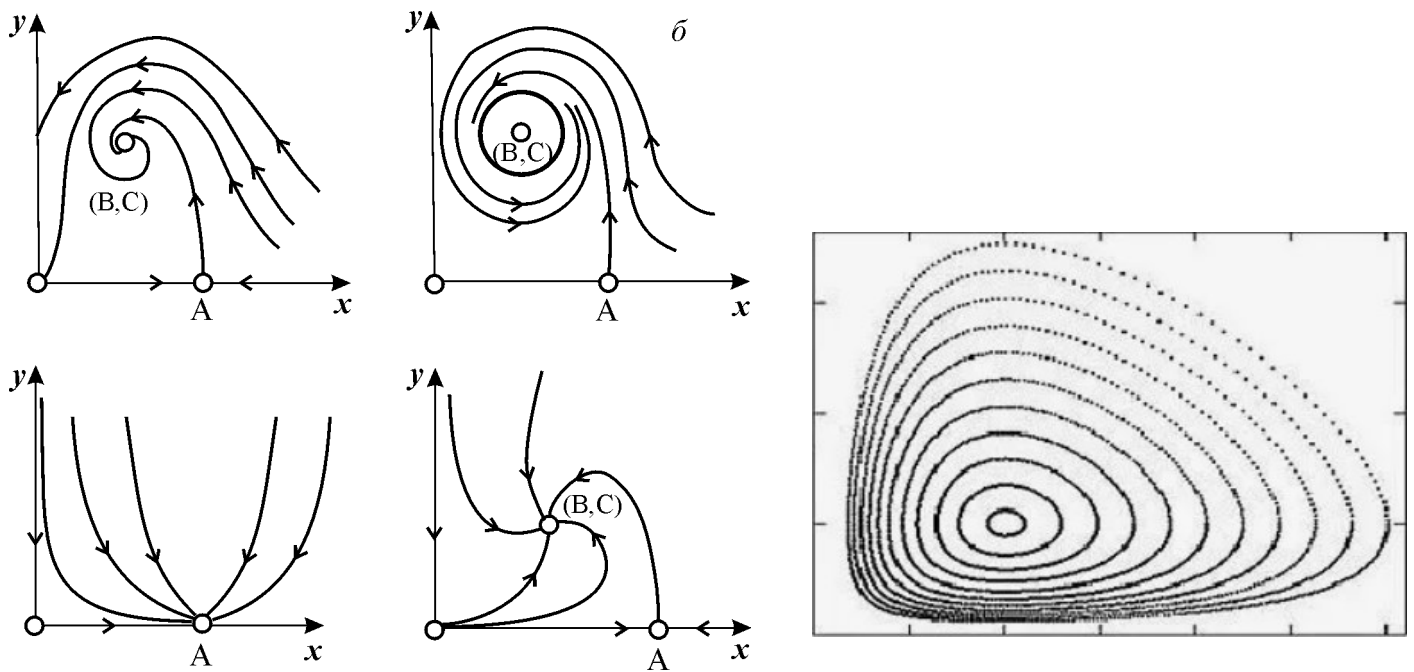
Figure 5. Visual representation of the Lotka-Volterra equations.
