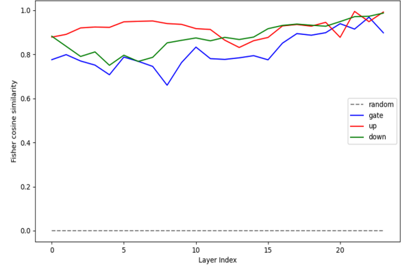
Figure 1 – Trace and Fisher similarity of the K-FAC matrices for sycophantic and truthful answers for gate_proj, up_proj and down_proj matrices of all the linear layers of Qwen2.5-0.5B-Instruct. The data shows that both tasks are located in the same valley of the loss-landscape but still treated differently.
