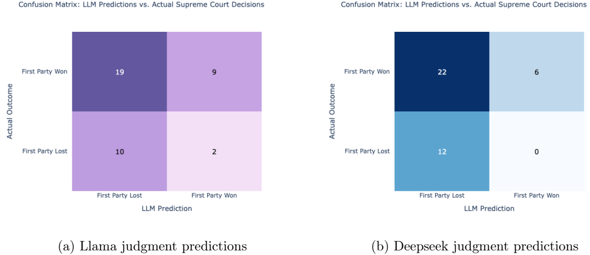
Figure 2: Confusion Matrices
